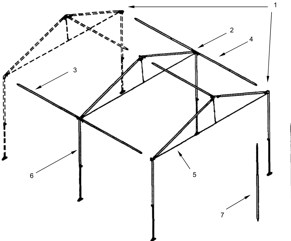
Figure 1. Frame Assembly.
